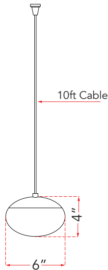
Front Elevation
